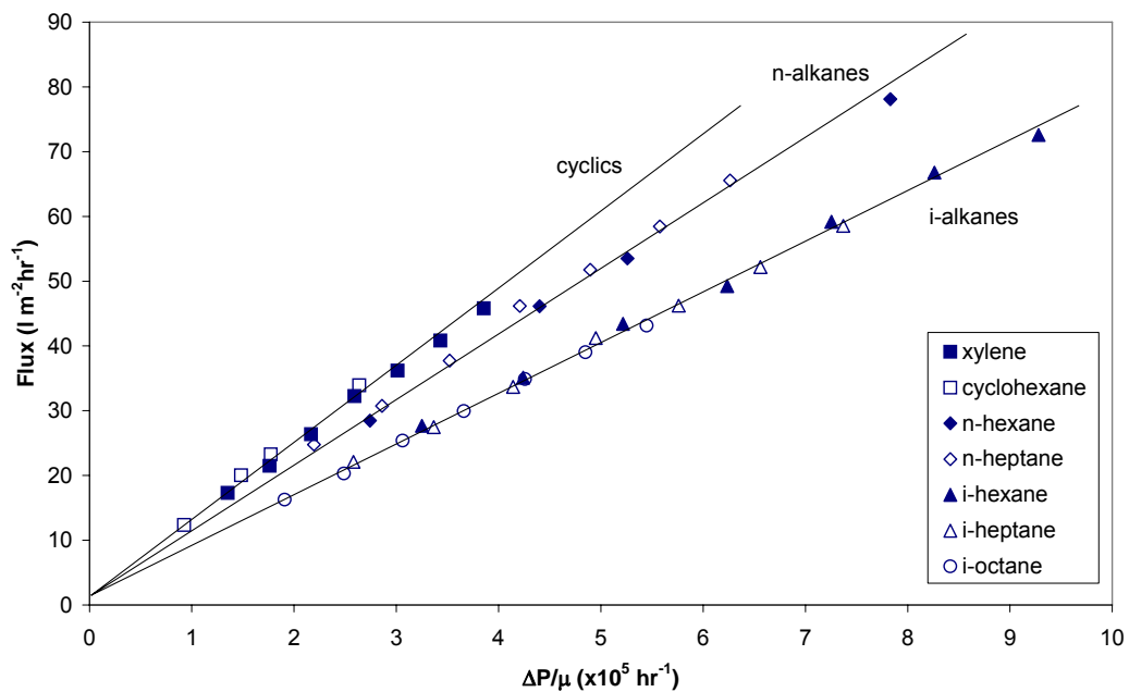
Figure 2: Solvent flux modelled with the Hagen-Poiseuille equation.
