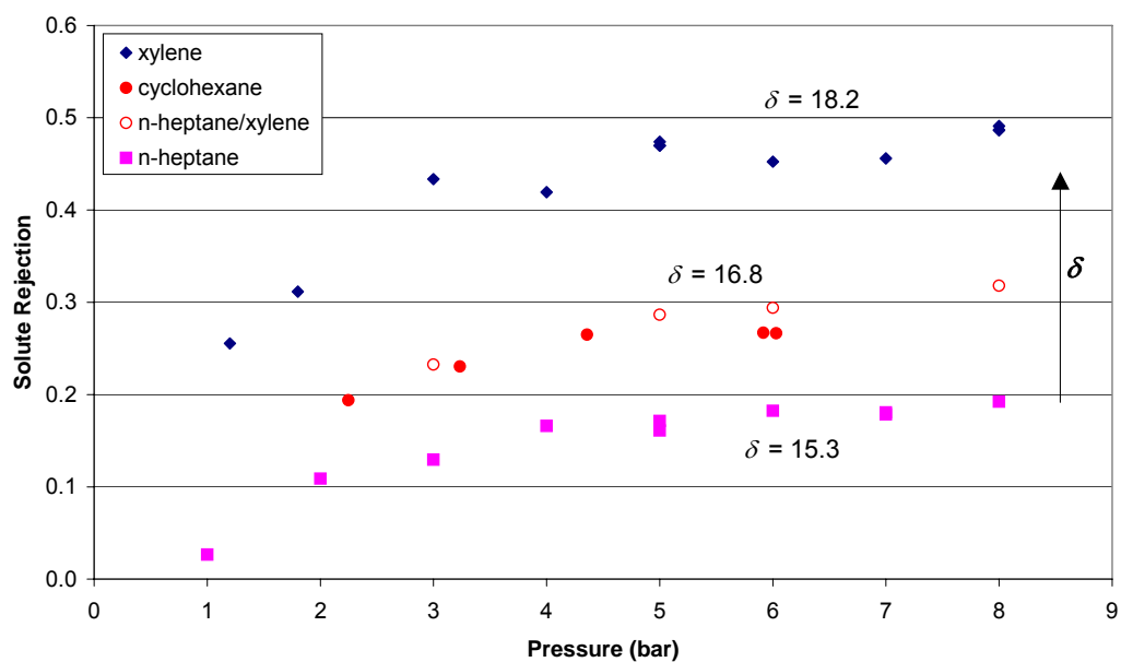
Figure 4: Effect of solvent-type ( \delta ) on solute rejection. n-heptane/xylene mixture has identical value of \delta to cyclohexane.
